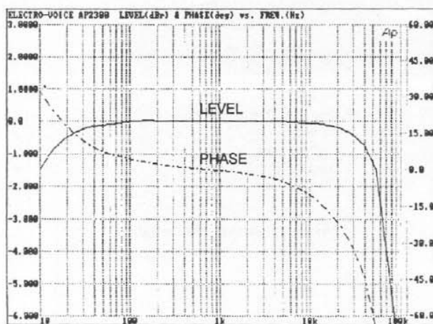
LEVEL + PHASE VS. FREQUENCY
